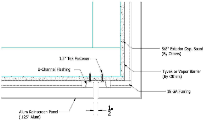
TYPICAL PANEL JOINT
